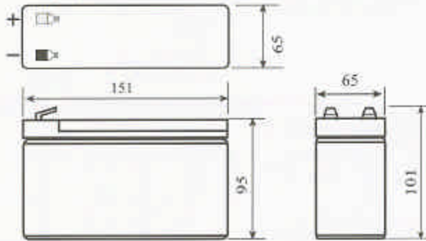
Dimensions (mm)
