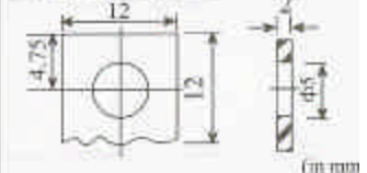
Optional Terminal B1-(copper) Bolt Type: M5
