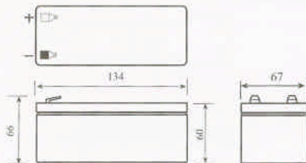
Dimensions (mm)
