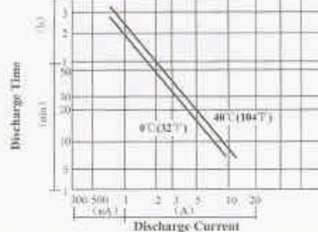
Discharge Characteristics (0°C/32°F, 40°C/104°F)
